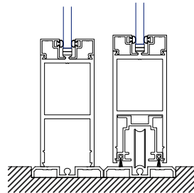
Recessed Tracks
