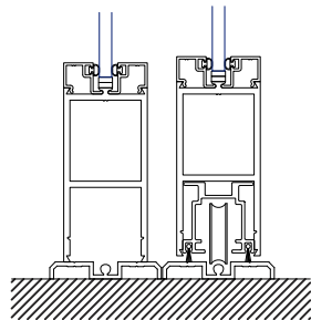
Surface Mounted Tracks
